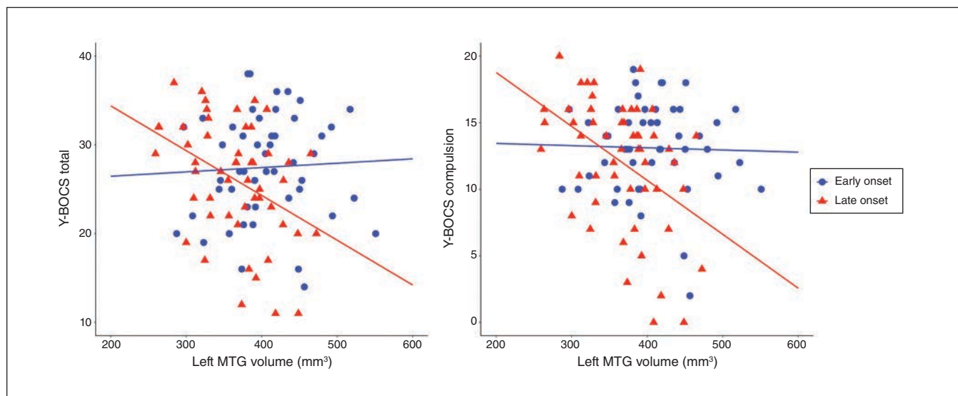
Fig. 2: Group \times volume interaction effect of the left middle temporal gyrus (MTG) on the severity of obsessive-compulsive symptoms across patients with early- and late-onset obsessive-compulsive disorder. Patients with a later onset and a smaller left MTG volume had higher total (left) and compulsion (right) scores on the Yale–Brown Obsessive Compulsive Scale. Y-BOCS = Yale–Brown Obsessive Compulsive Scale.
