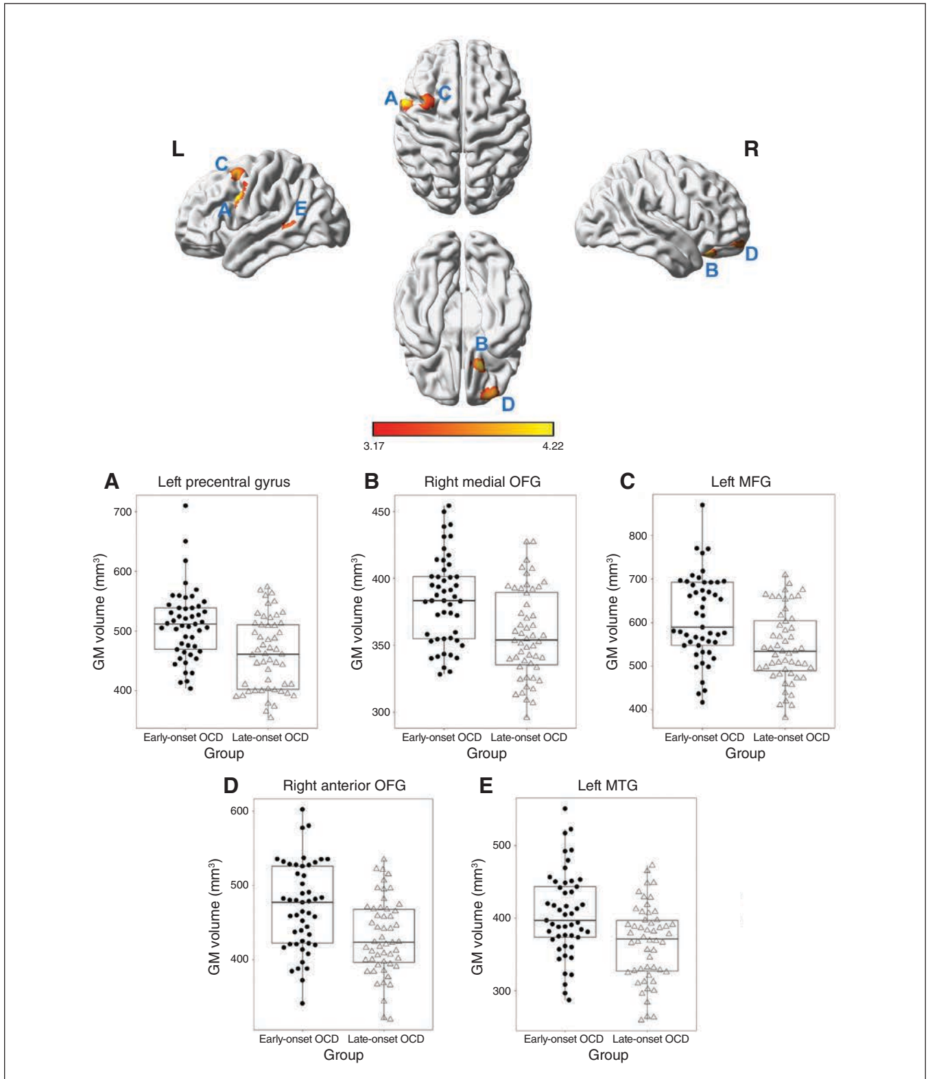
Fig. 1: Structural differences in grey matter volumes between patients with early- and late-onset obsessive–compulsive disorder (OCD). Top: Brain regions that were significantly larger in early-onset OCD than in late-onset OCD; these regions included (A) the left precentral gyrus, (B) the right medial orbitofrontal gyrus (OFG); (C) the left middle frontal gyrus (MFG); (D) the right anterior OFG; and (E) the left middle temporal gyrus (MTG). Bottom: plots showing significantly larger regional grey matter (GM) volumes in early-onset OCD than in late-onset OCD.
